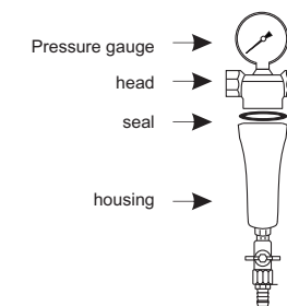
Fig.1 FHMB filter parts
